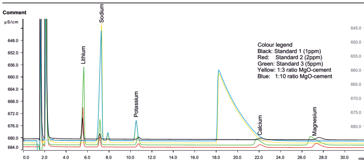
Figure 12. Selected cations content for leaching study (calcium and magnesium) by ion chromatography using a conductivity detector.
