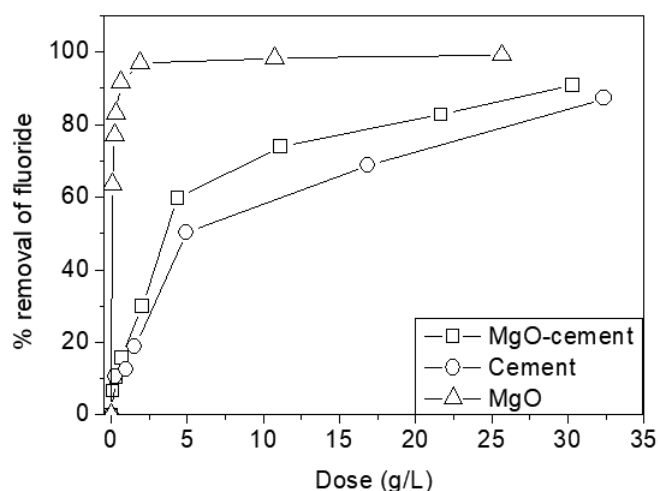
Figure 1. Dose effect on fluoride removal.
