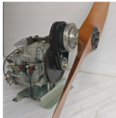
Photo: 65 hp Rotary engine developed by VRDE
