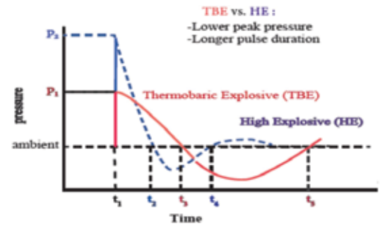
Comparison of Thermobaric and High Explosive
