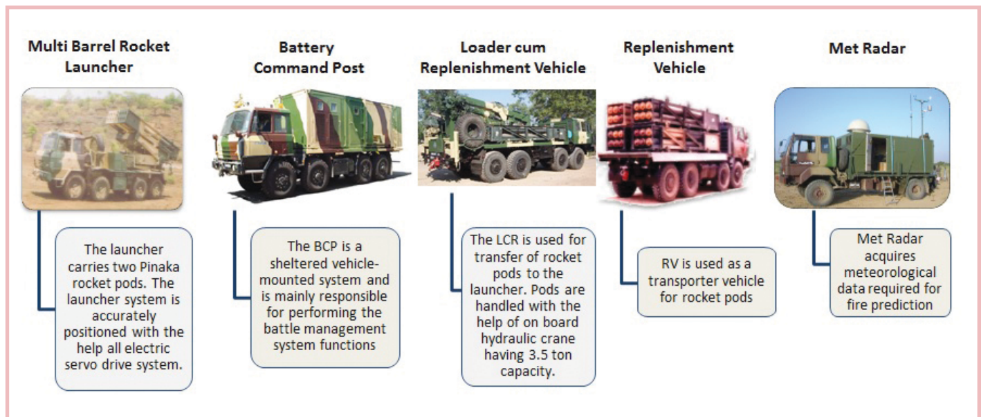
Components of Pinaka Battery
