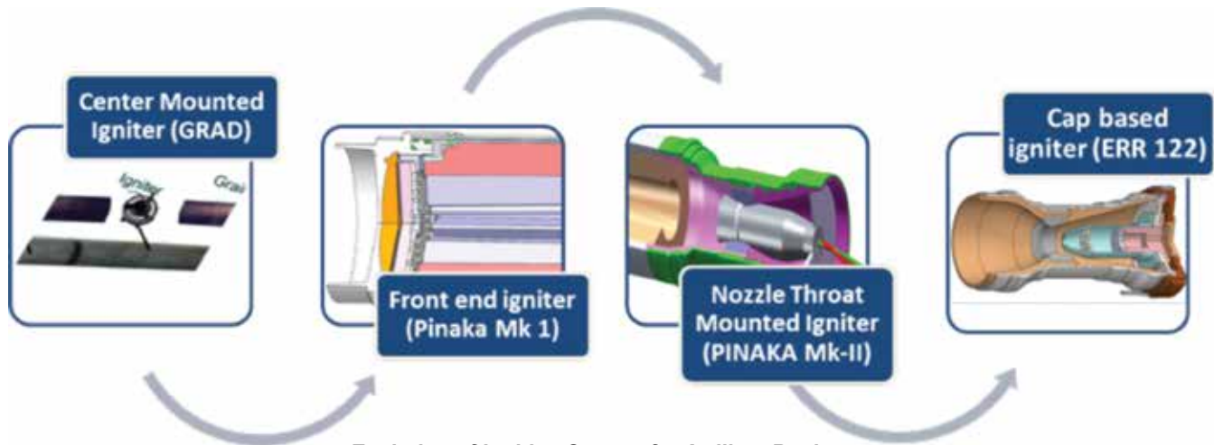
Evolution of Ignition System for Artillery Rockets
