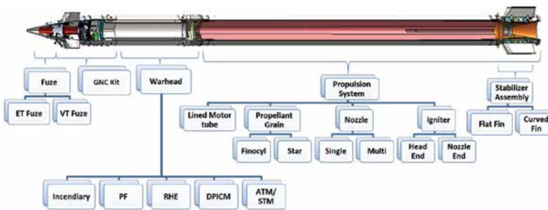
Components of Typical Artillery Rocket
