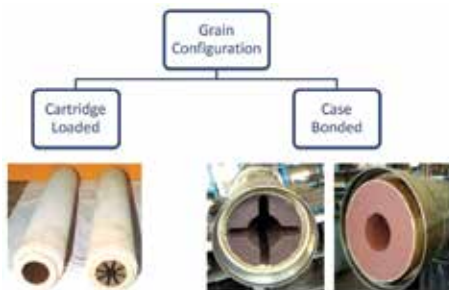
Cartridge loaded and case bonded grains
