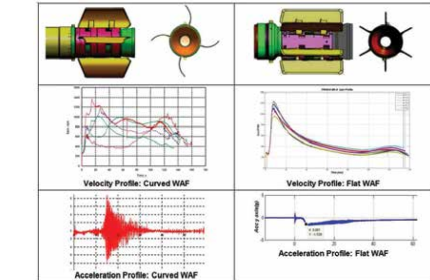
Stabilizer Redesign to Overcome High Mach Number Dynamic Instabilities (from curved Wrap Around Fin to Flat Wrap Around Fin stabilizer)
