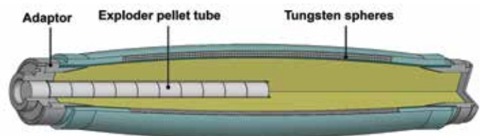
Sectional View of PF Warhead Module
