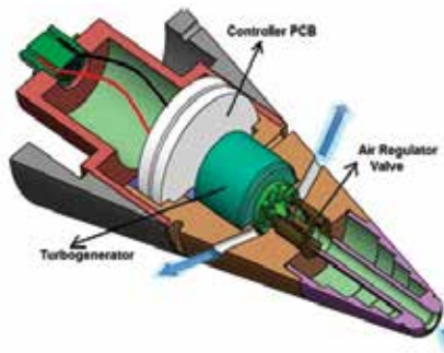
ET Fuze with Turbo Generator
