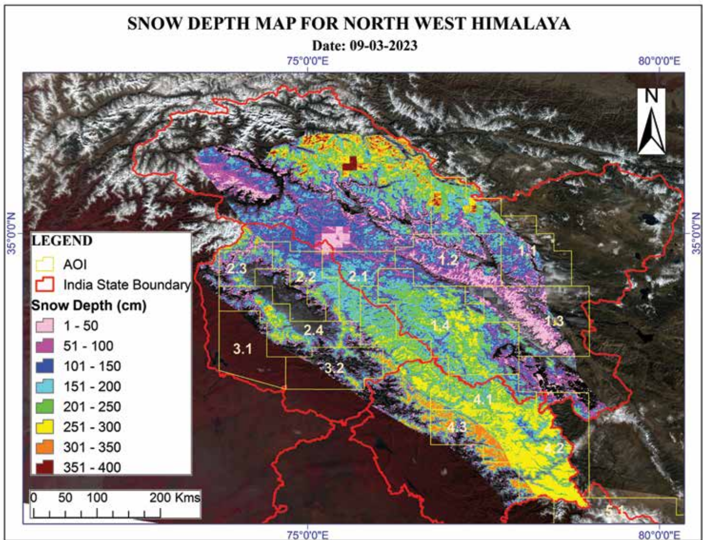
Figure 5. Snow-depth Distribution in North-West Himalaya.
