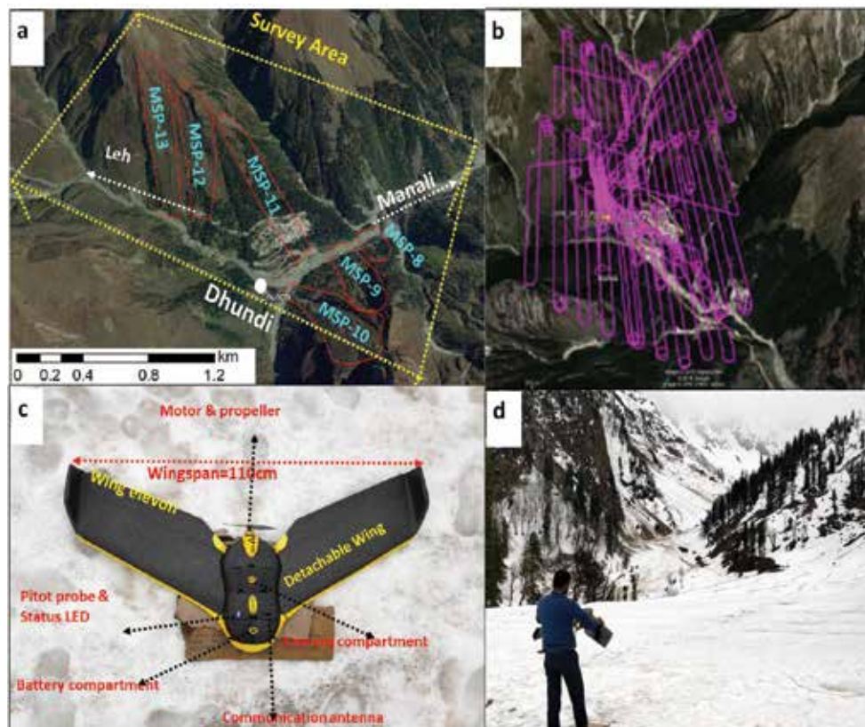
Figure 7. (a) UAV Survey Area Covering Major Avalanche Sites (MSP (Manali South Portal)-8 to MSP-13) Near Dhundi Region, (b) Winter Survey Flight Path of UAV, (c) Schematic of the e-Bee X UAV with Labels Indicating Sensors and Major Components and (d) Field Photograph of Launching UAV by Hand.
