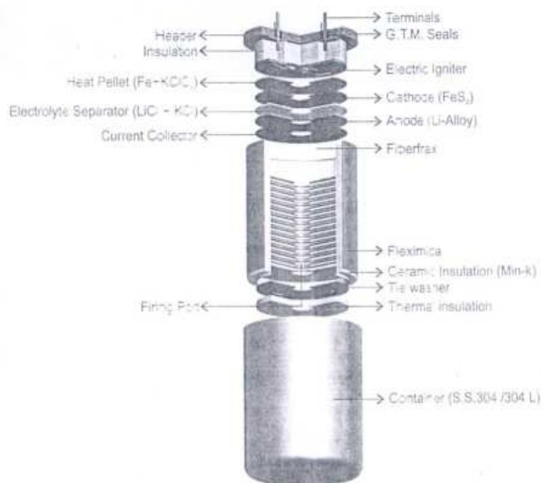
Figure 5-12 Typical Thermal Battery Features supplied by M/s H.B.L Hyderabad
