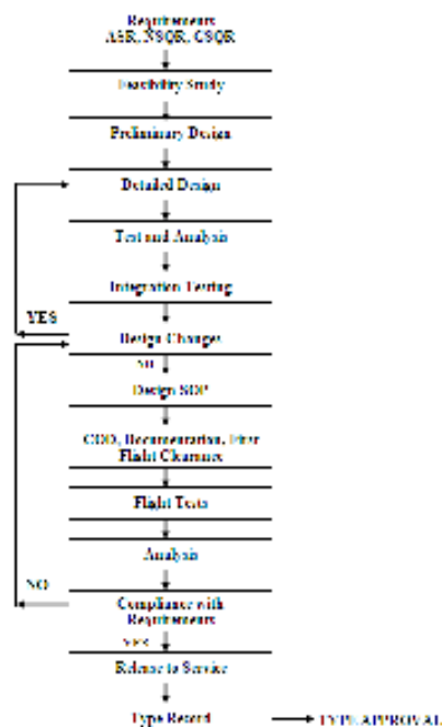
Figure 7-1 Airworthiness flow chart
