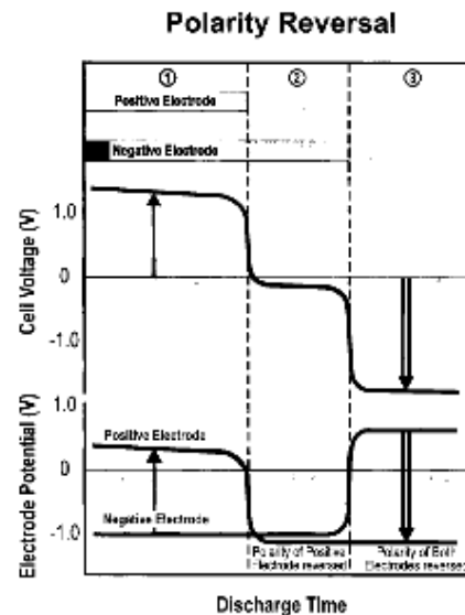
Figure 3-31 Polarity reversal
