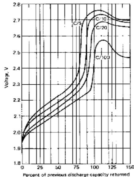
Figure 3-62 Voltage curves for batteries charged at various constant-current rates at 25°C.
