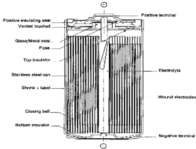
Figure 4-2 Cutaway view of lithium/thionyl chloride spirally wound electrode battery.
