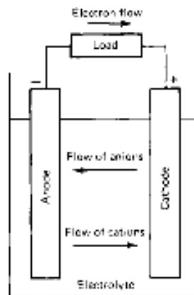
Figure 1-6 Electrochemical operation of a cell (discharge)
