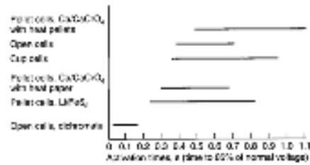
Figure 5-8 Activation times of different thermal battery cell designs.
