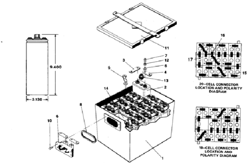
Figure 3-10 Typical Battery Assembly
