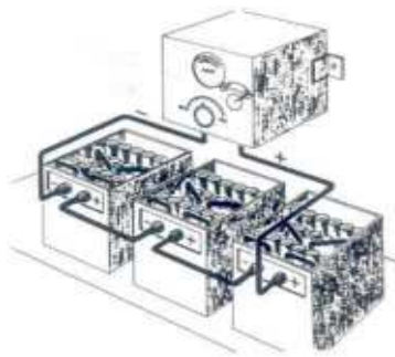
Figure 3-61 Constant current charging
