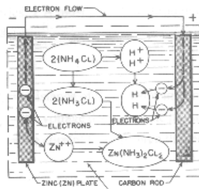
Figure 1-4 Chemical action in a voltaic cell
