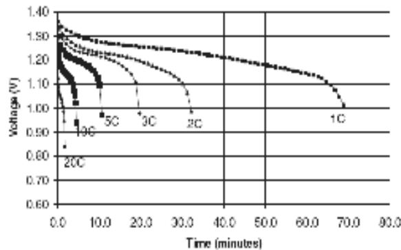
Figure 3-15 Typical discharge curves at various C rates, 25°C.
