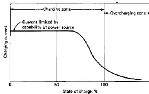
Figure 3-24 Constant-potential charge current
