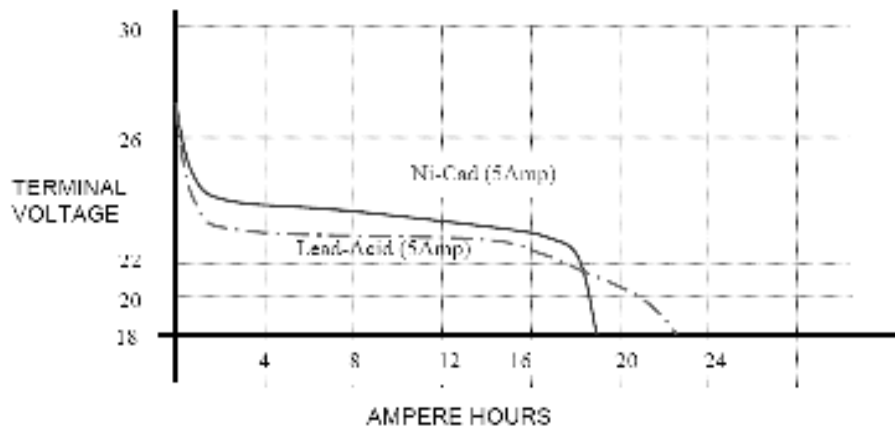
Figure 2-4 Typical discharge rates of Lead acid and Nickel cadmium batteries
